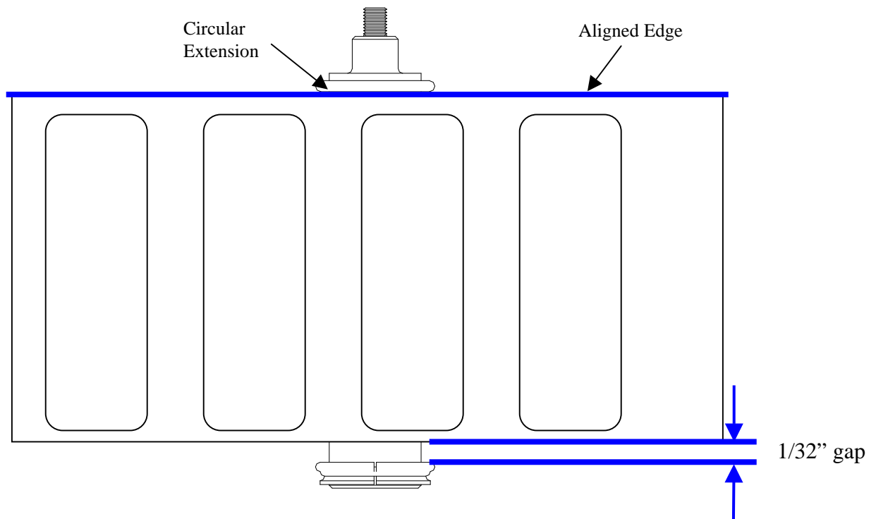
Figure 3-12: Gap between backer material and Tab Backer Guide.
