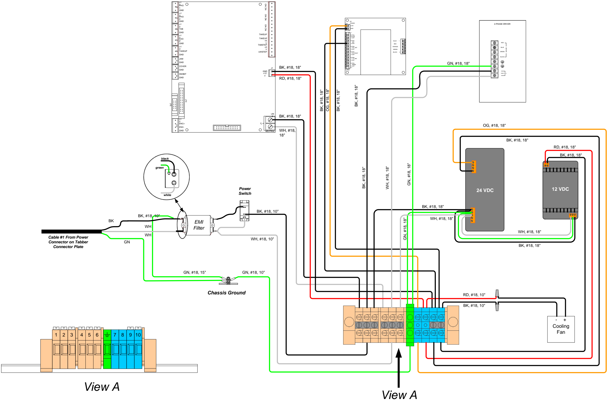
Figure B-9: BK731-2 Tabber Head Wiring - Page 2 of 6
