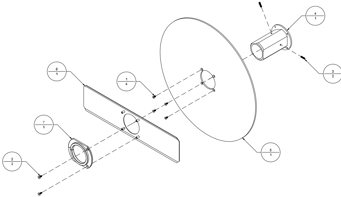
Figure A-25: Unwind Disc Assembly (9101145A)
