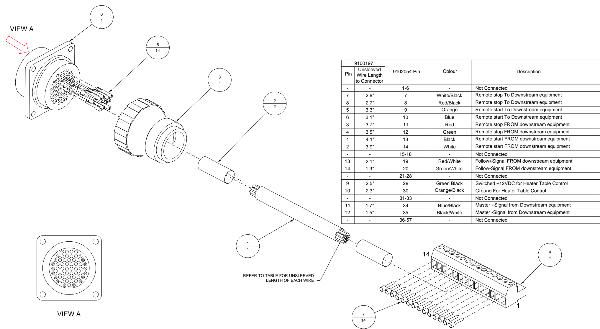
Figure A-50: Cable, Downstream to BCB (9104144A)
